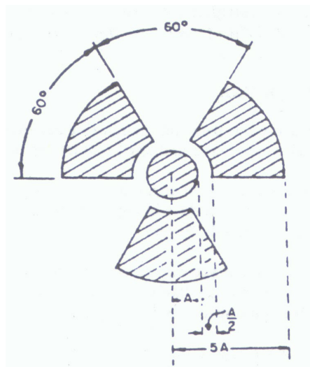
RADIATION SYMBOL
